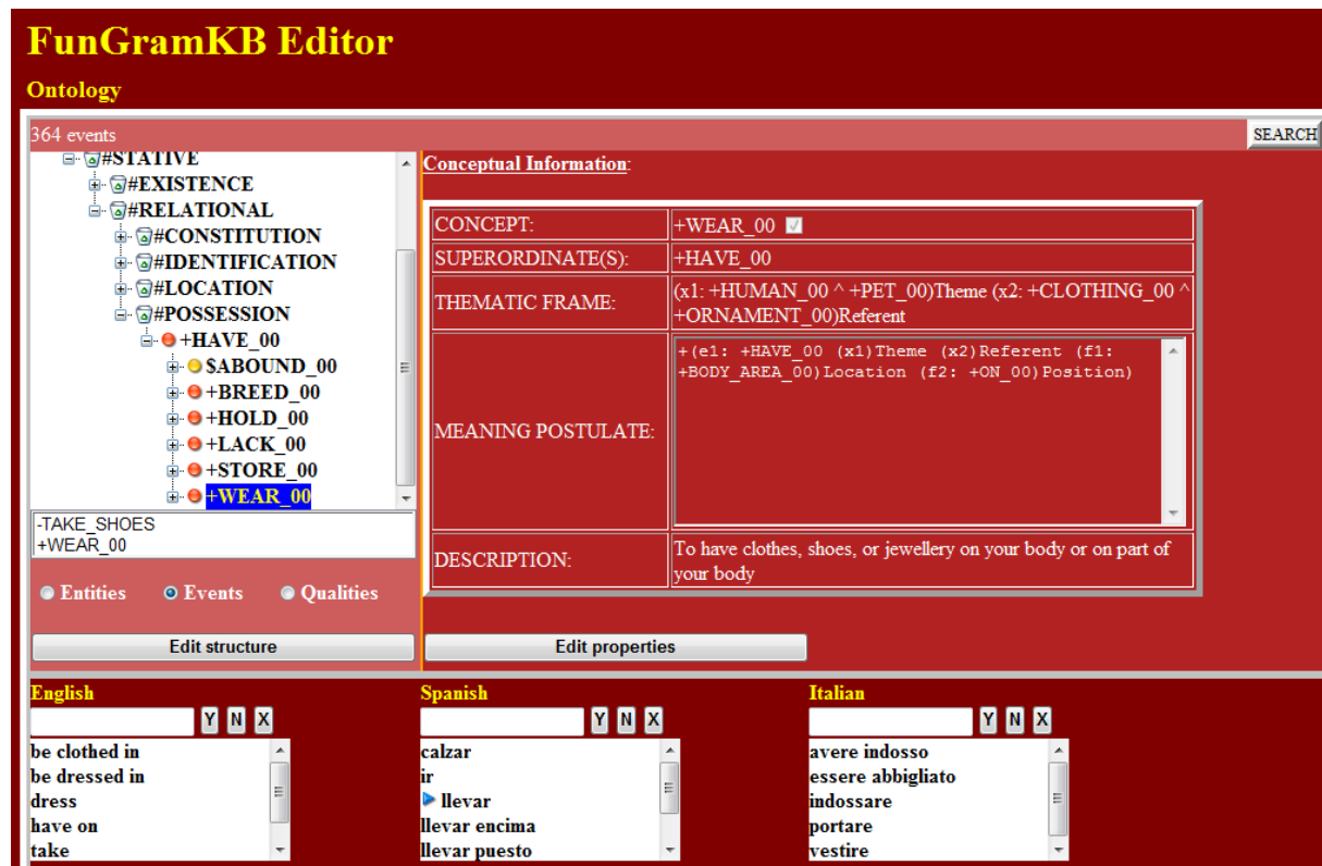
Fig. 3. Ontological information of +WEAR_00.
